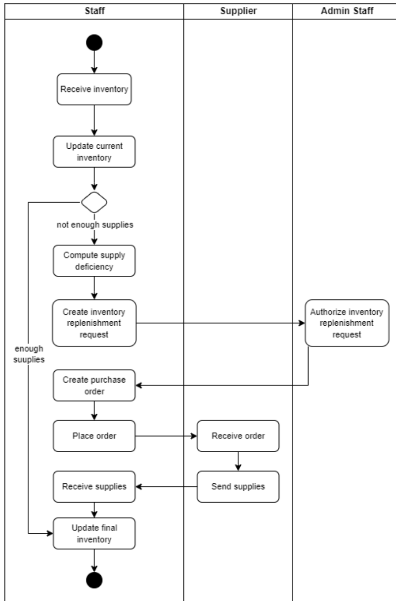
Figure 5.7.2 Proposed Inventory Activity Diagram
