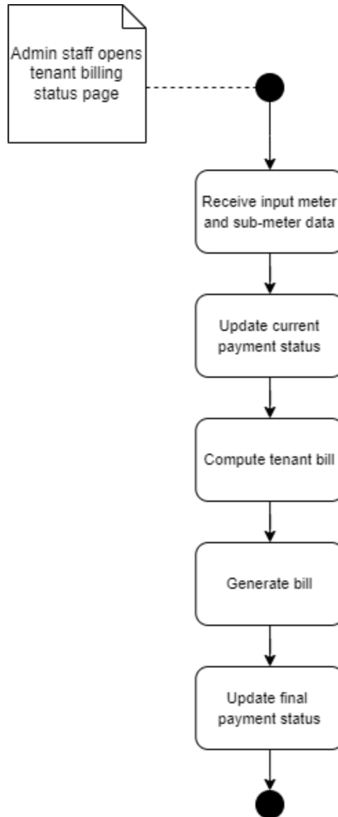
Figure 5.7.3 Proposed Tenant Billing Activity Diagram
