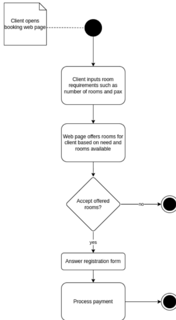
Figure 5.7.1 Proposed Booking Activity Diagram
