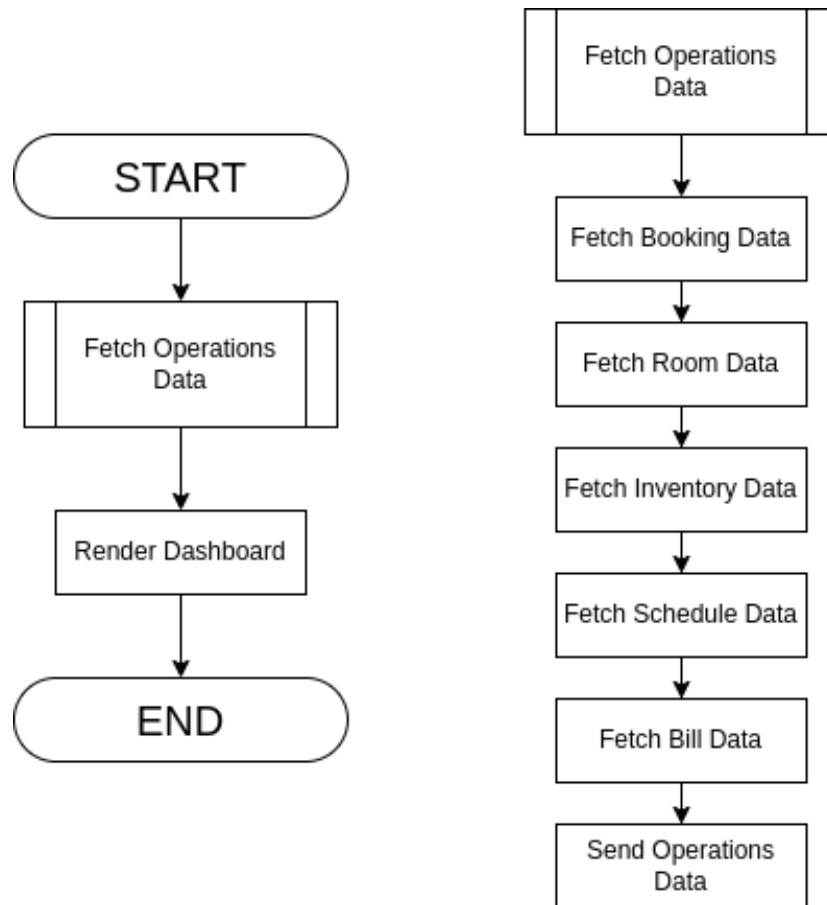
Figure 5.1.5 Proposed Dashboard PFD
