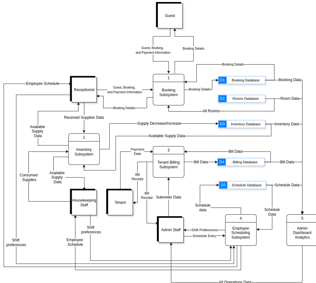
Figure 5.2.1 Proposed DFD for RCMIS
