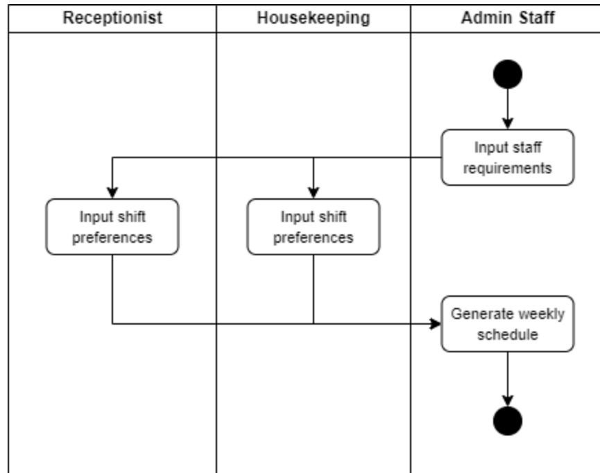
Figure 5.7.4 Proposed Employee Scheduling Activity Diagram
