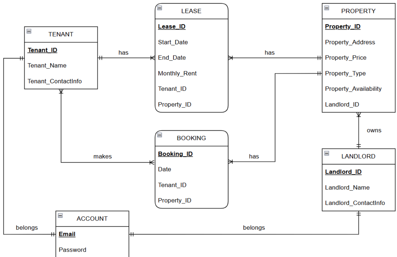
Figure 1.2 Commercia Entity Relationship Diagram (ERD)
