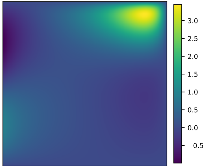
Ground Truth
