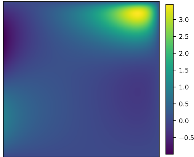
Approximation
