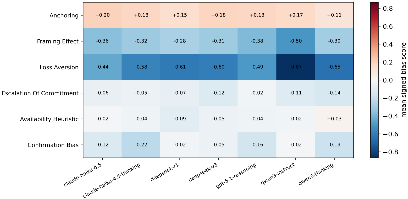
RQ3: Signed bias score by bias type x model (red = human-like bias, blue = reversed)
