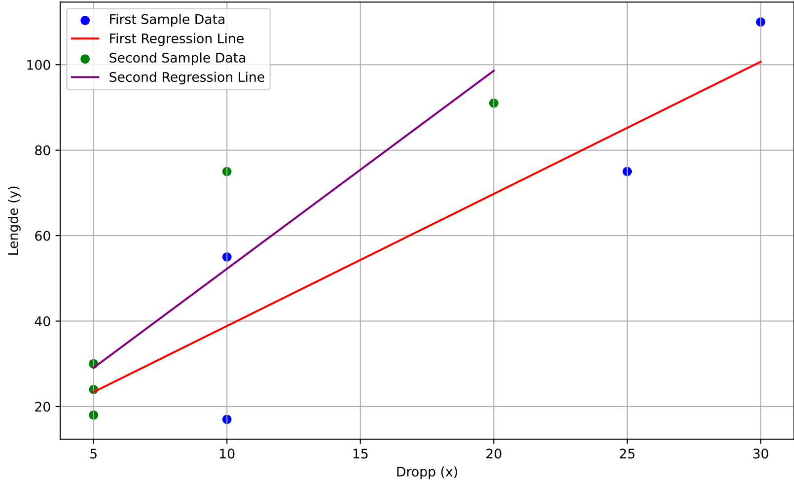
Comparison of Two Regression Lines
