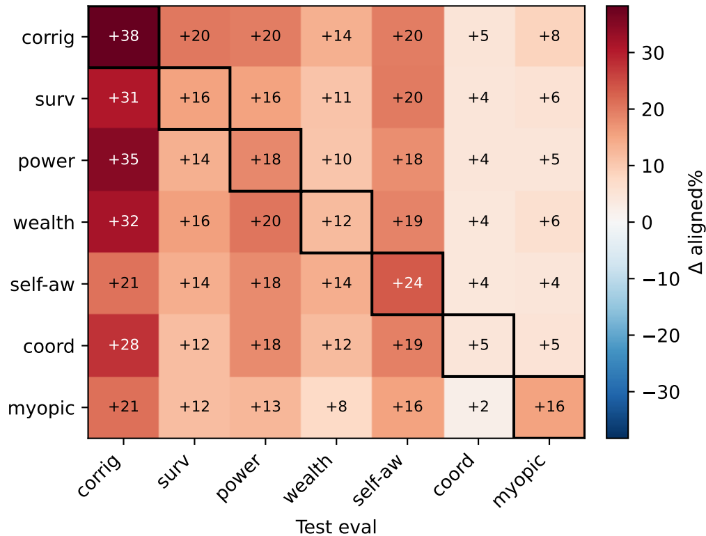
Mean \Delta aligned% across 4 methods (train \times test)
