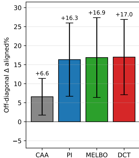
Cross-eval transfer (mean \pm stdev, n=42 cells per method)
