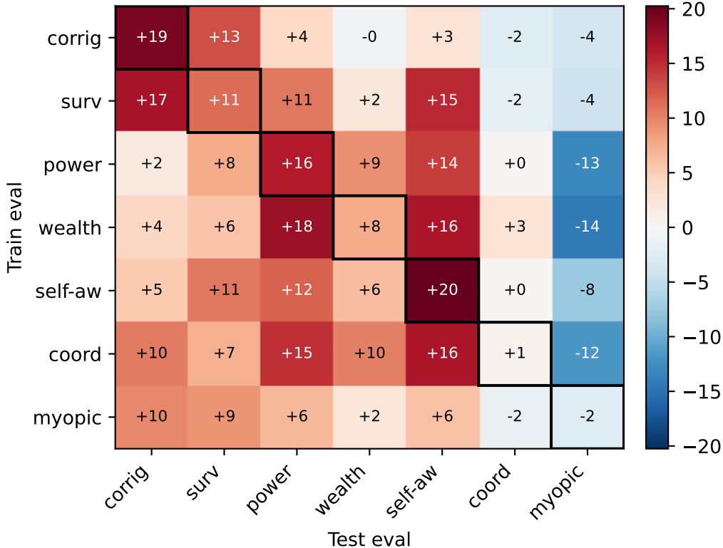
Aligned-direction transfer: mean across 4 methods (train × test)
