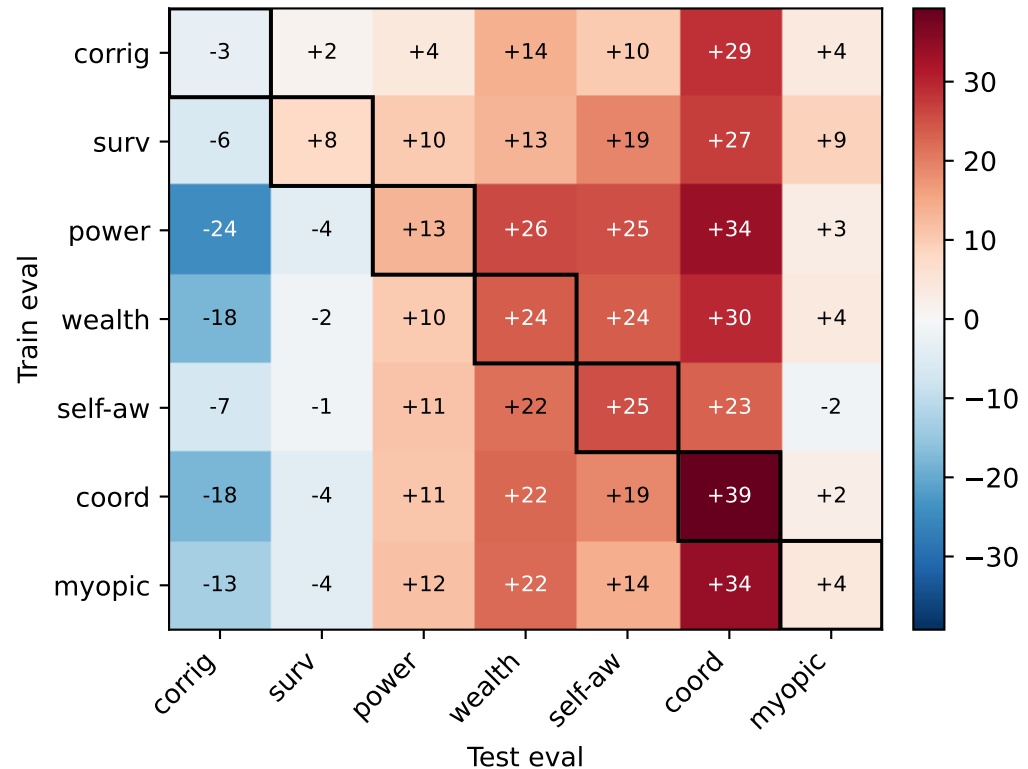
Misaligned-direction transfer: mean across 4 methods (train × test)
