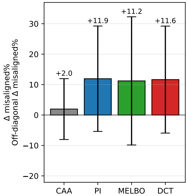
Cross-eval misaligned transfer (mean ± stdev, n=42 cells per method)
