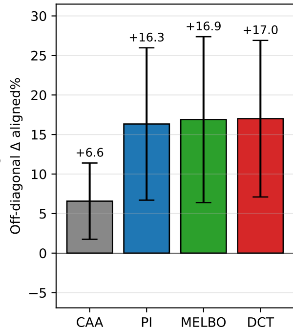
Cross-eval aligned transfer (mean ± stdev, n=42 cells per method)
