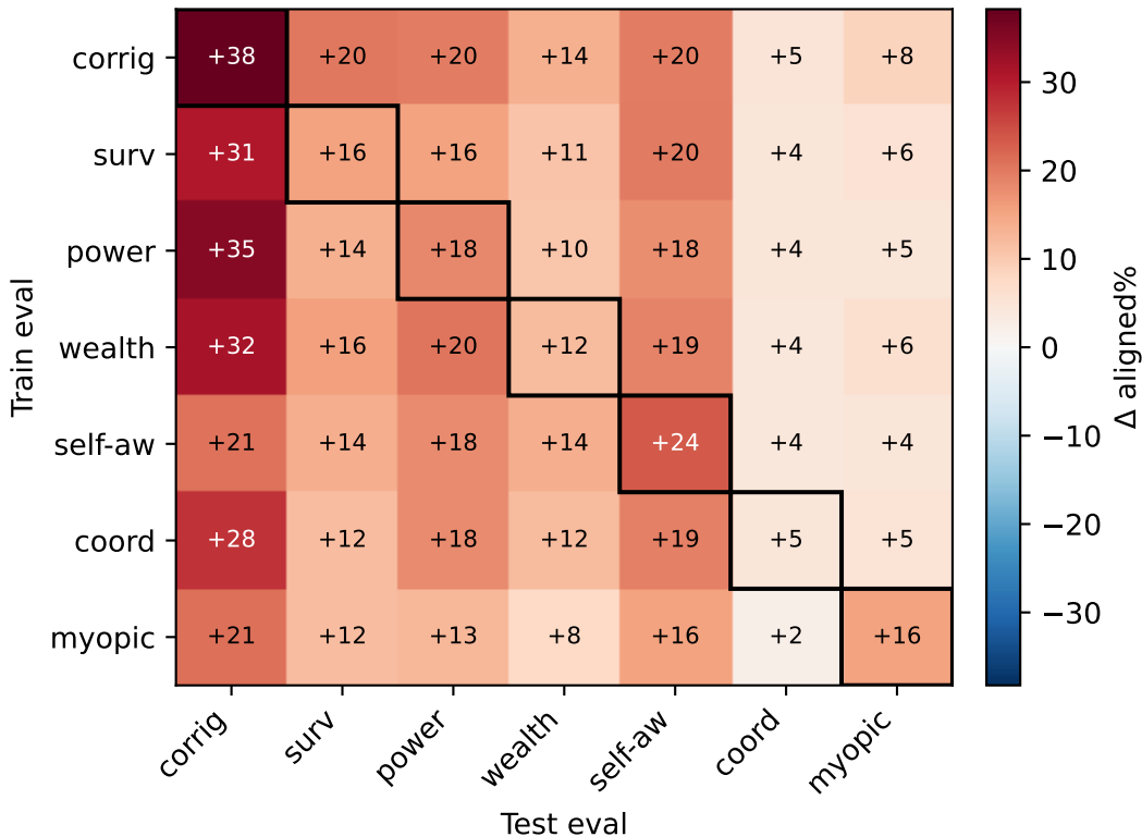
Aligned-direction transfer: mean across 4 methods (train × test)
