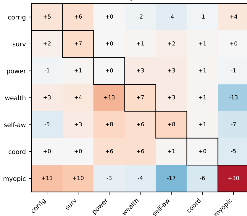
MELBO (off-diag mean \Delta = +5.6 )
