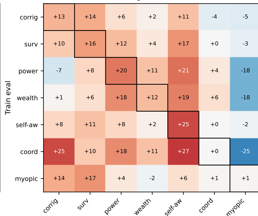
DCT (off-diag mean \Delta = +7.9 )
