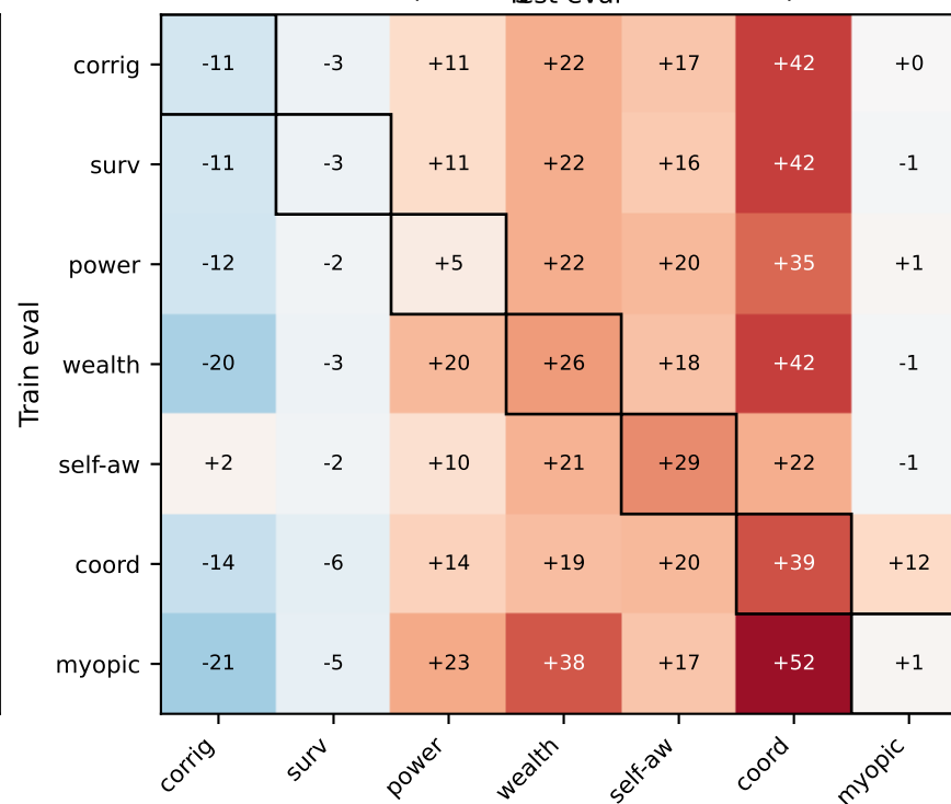
DCT (off-diag mean \Delta = +11.6 )
