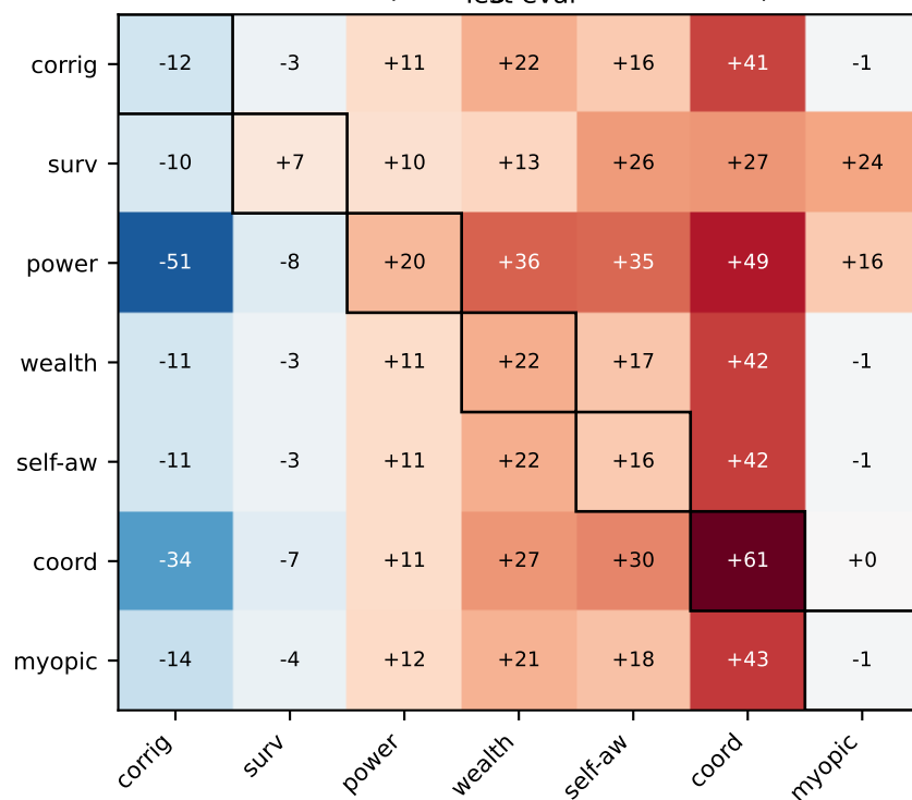
MELBO (off-diag mean \Delta = +11.2 )
