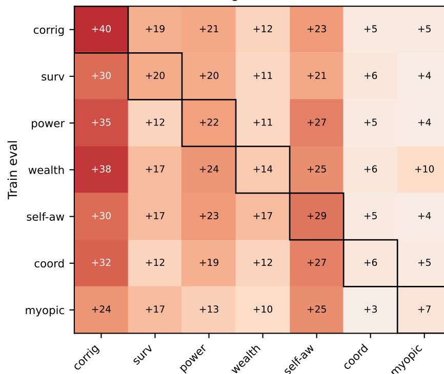
DCT (off-diag mean \Delta = +17.0 )
