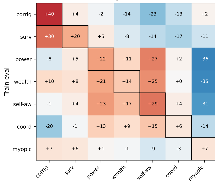
DCT (off-diag mean \Delta = +2.8 )
