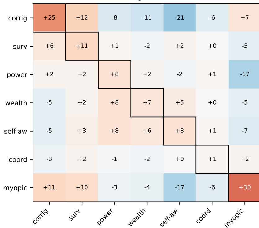
MELBO (off-diag mean \Delta = -0.6 )
