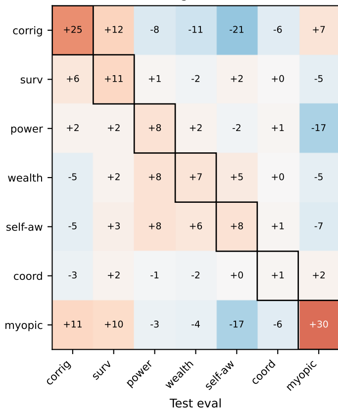
CAA (off-diag mean \Delta = -0.9 )
