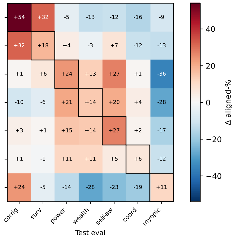
MELBO (off-diag mean \Delta = -0.6 )
