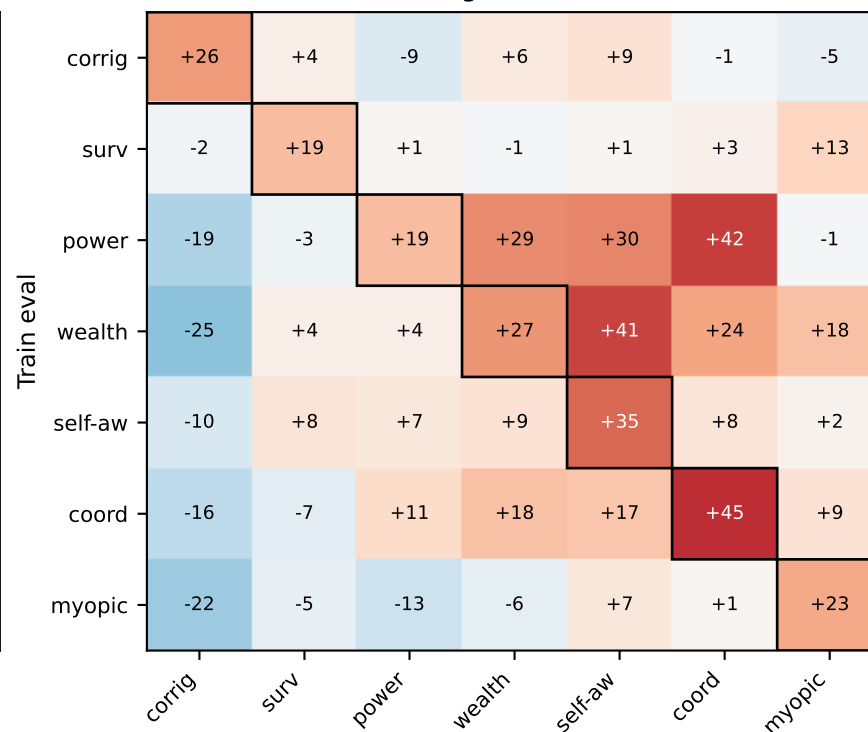
DCT (off-diag mean \Delta = +1.3 )
