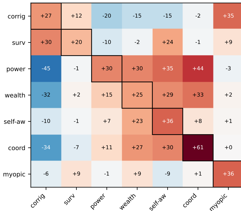
MELBO (off-diag mean \Delta = +5.0 )
