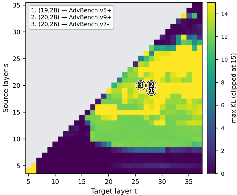
Refusal-phishing KL atlas (Qwen3-14B) 396/560 active pairs (max-KL \geq 0.5 )
