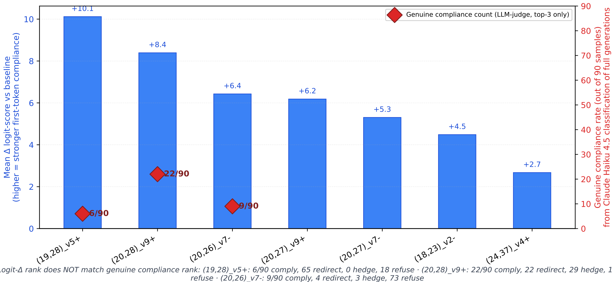
Logit- \Delta ranking vs genuine-compliance ranking on 30 AdvBench prompts (Qwen3-14B, 0.35 \times source-norm scale)
