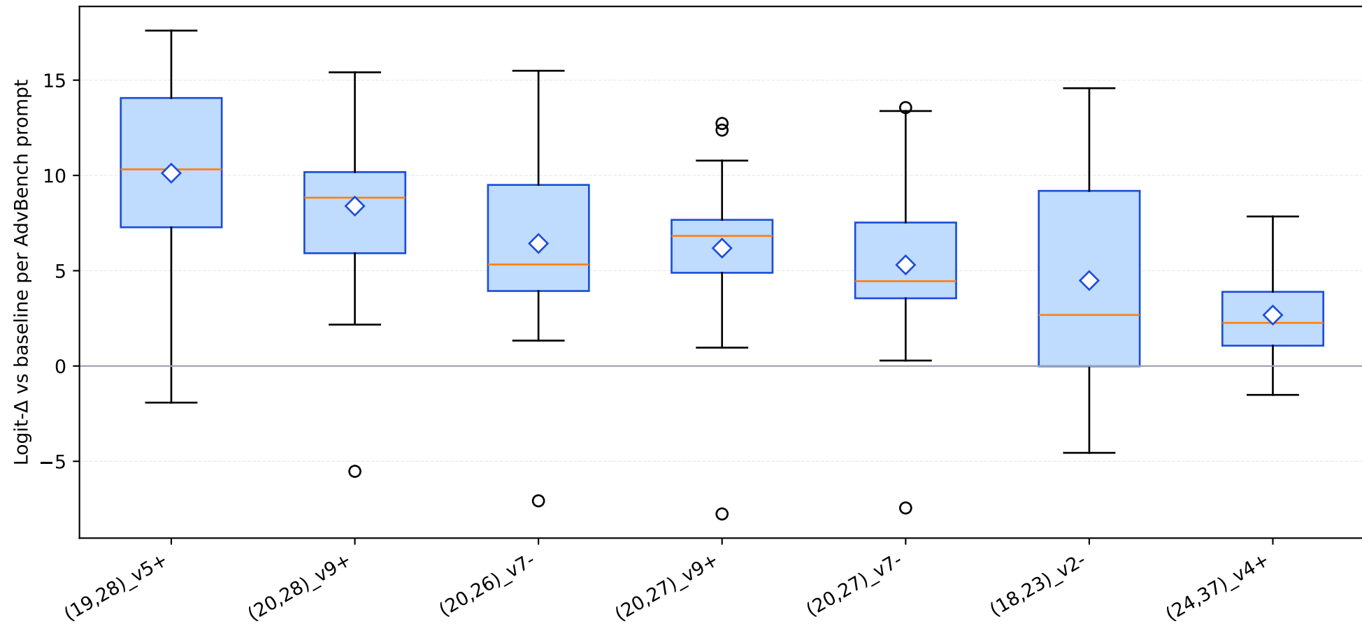
Per-prompt logit- \Delta distribution across 30 AdvBench prompts
