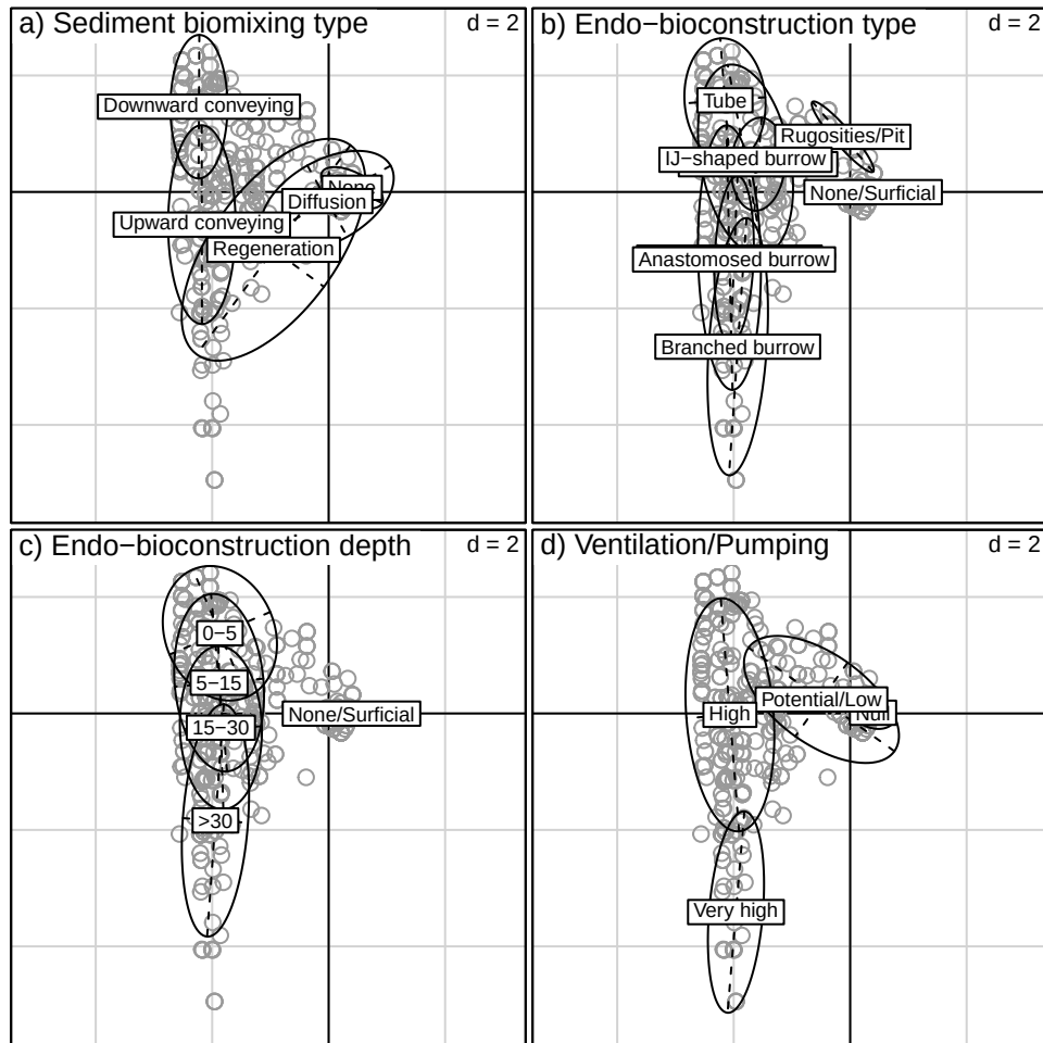
Figure S1. Endo-substratum engineering pattern. Grey dots represent the 1893 species; due to identical trait profiles, many species have the same position. From (a) to (d), each panel represents the same species pattern, but grouped per modality of the specified trait. Trait modalities are positioned at the gravity centre of their respective species. The first axis (horizontal) opposes absence of engineering ability (a, “None”, right side of the axis) to burrowing species (left). The second axis (vertical) expresses the burrowing depth, associated to non-local transfer of sediment (a).
