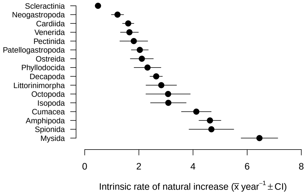
Figure S5. Intrinsic rate of natural increase in various orders. Each order comprises a minimum of 30 species.
