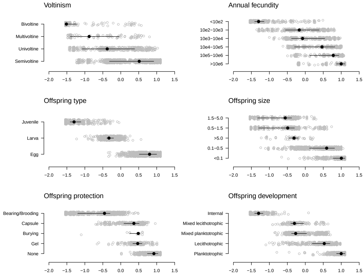
Figure S3. Reproductive and developmental trait modality distributions along the first axis of Fuzzy Correspondence Analysis.
