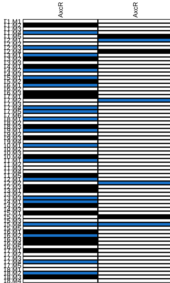
Figure S13. Significance tests of correlations between trait modalities and RLQ axes (right, first axis; left, second axis). White, not significant ( p \geq 0.05 ); blue, significant and positive correlation; black, significant and negative correlation.
