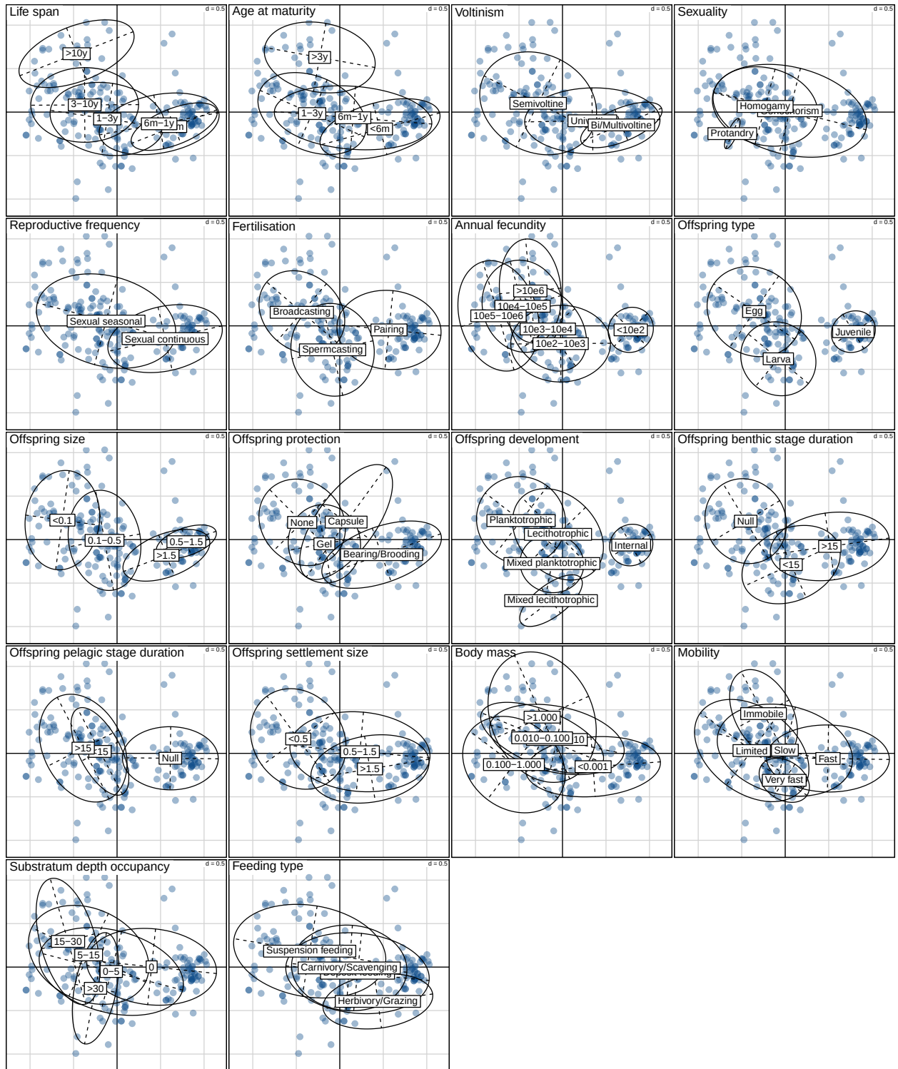
Figure S14. RLQ analysis of the high dynamics habitat, trait representation along axis 1 (horizontal) and 2 (vertical). Each panel represents the same species pattern (blue dots) group by their respective modalities of the considered trait.
