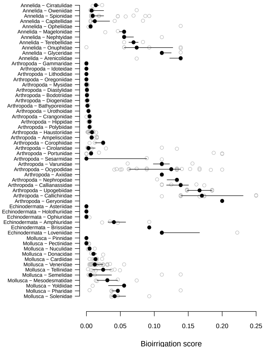
Figure S9. Total bioirrigation score per family. Grey dots, species; black dot, mean; bars extend from 25th to 75th percentile.
