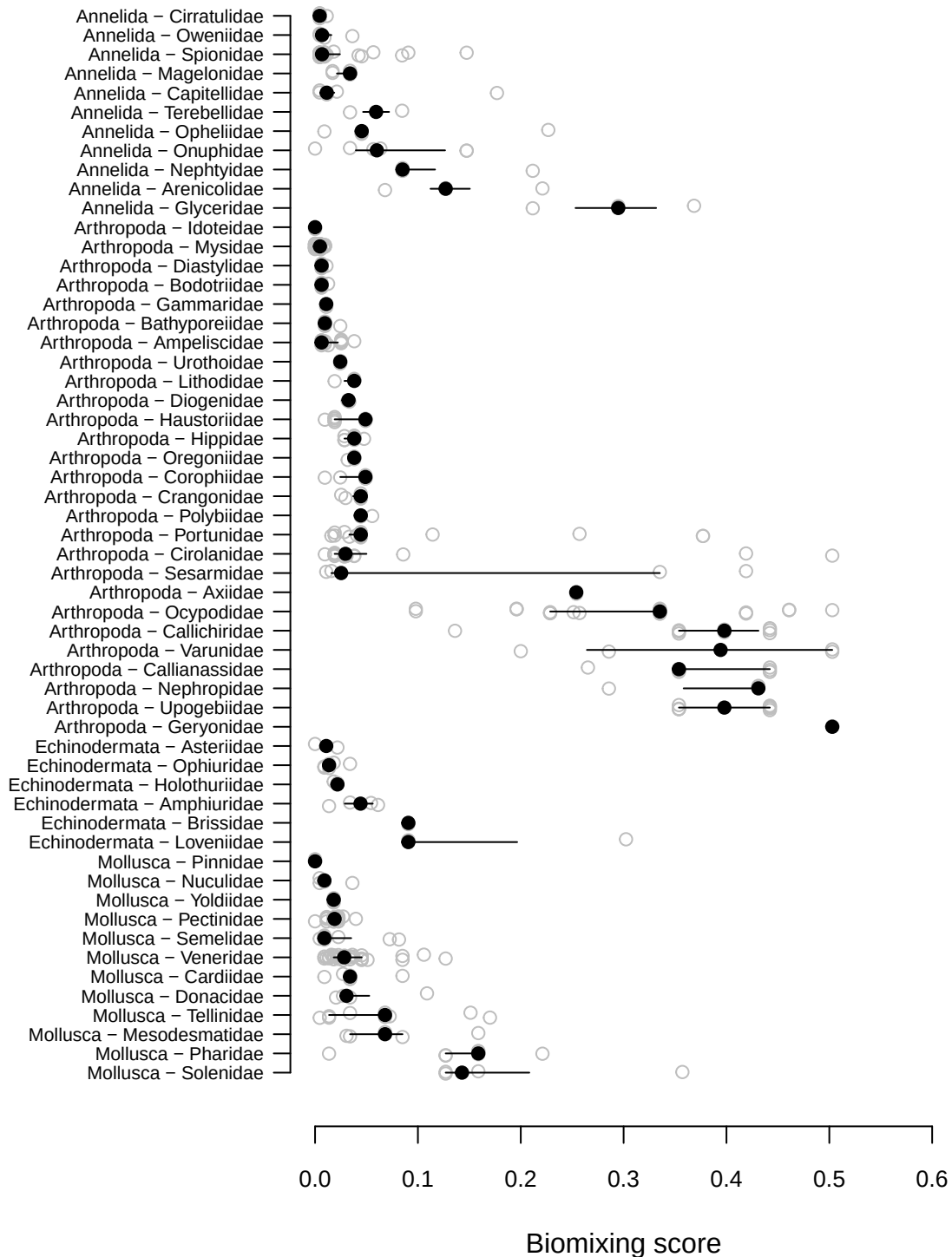
Figure S8. Total biomixing score per family as the product of the four individual biomixing types (biodiffusion, upward conveying, downward conveying and regeneration). Grey dots, species; black dot, mean; bars extend from 25th to 75th percentile.
