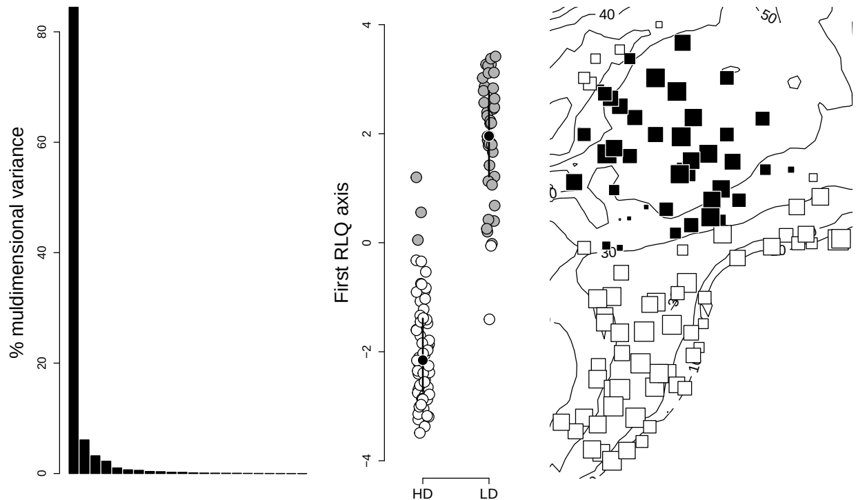
Figure S10. RLQ analysis of the whole area. Left panel, eigenvalue diagram showing a prominent first axis. Middle, sampling station first axis scores showing the distinction between high and low dynamics habitats (HD and LD, respectively; black dot, median score; bars extend from 25th to 75th percentiles). Right, sampling axis scores mapped over the area; black, positive scores; white, negative scores; square size proportional to deviation from 0. Contour lines, depth in meters.
