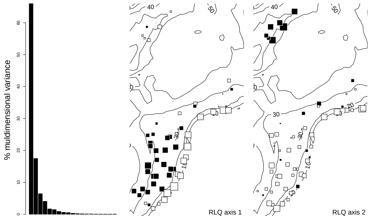
Figure S12. RLQ analysis of the high dynamics habitat. Left panel, eigenvalue diagram showing two axes that deserve interpretation. Middle and right, mapping of sampling station first and second axis scores, respectively. Black, positive scores; white, negative scores; square size proportional to deviation from 0. Contour lines, depth in meters.
