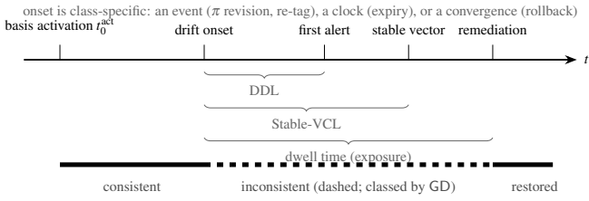
Fig. 4. The drift lifecycle and its temporal quantities (Definition 9). Substantive onset is episode- and class-specific—an organizational event (policy revision), a clock crossing (exception expiry), an exogenous event (registry re-tag), or reconciler convergence (rollback); evidence onset is the distinct transition of a required mask entry to zero. Drift detection latency (DDL; Metric M2) ends at the first honest alert; stable vector-completion latency (Stable-VCL; Metric M2) ends only when an admissible cut is closed by the required watermarks. Without that closure Stable-VCL is censored. Substantive and evidence dwell are reported separately; their remediation families are also distinct (Section IV-C).
