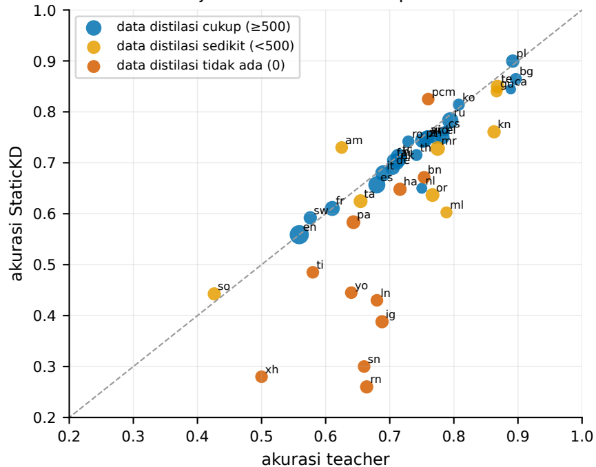
Set uji: StaticKD vs teacher per bahasa
