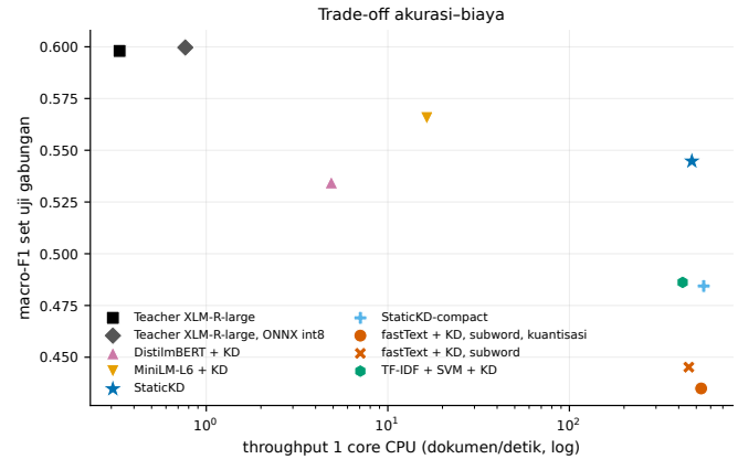
Gbr. 6. Trade-off macro-F1 set uji gabungan terhadap throughput satu core CPU (skala log).
