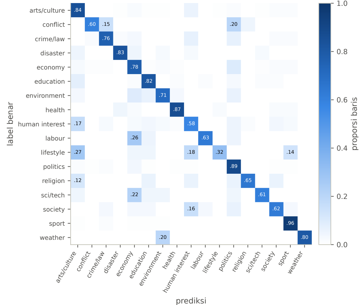
StaticKD: confusion matrix ternormalisasi (dev)
