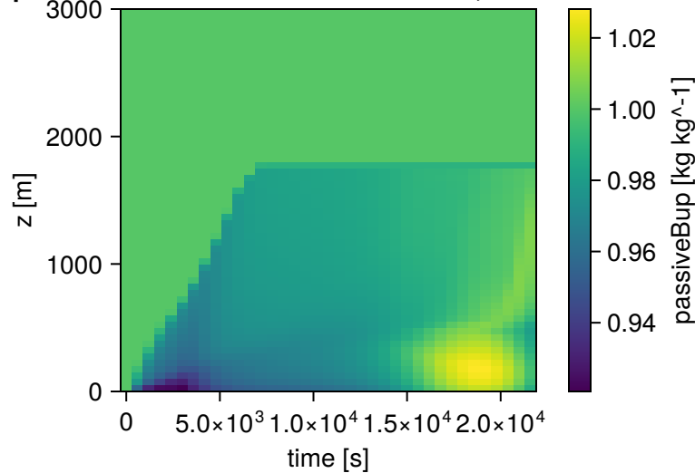
Updraft Passive Tracer B Concentration, Instantaneous
