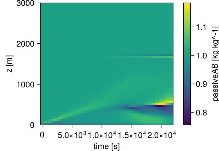
Passive Tracer AB Concentration, Instantaneous
