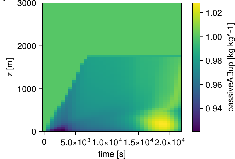
Updraft Passive Tracer AB Concentration, Instantaneous
