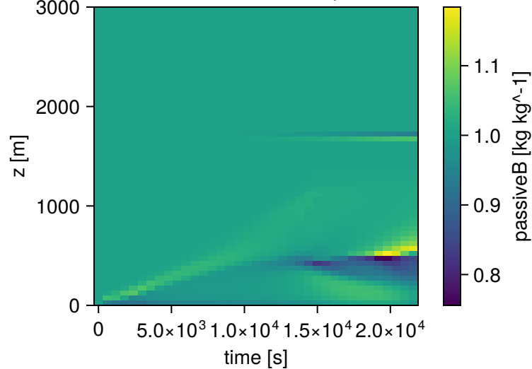
Passive Tracer B Concentration, Instantaneous
