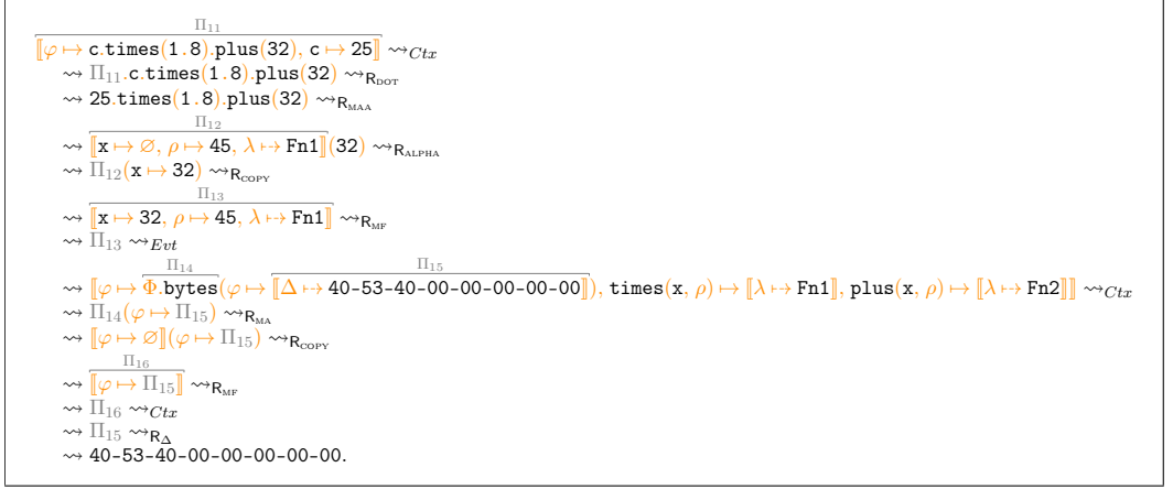
Fig. 8. Dataization of Eq. (6), generated by phino 0.0.142.
