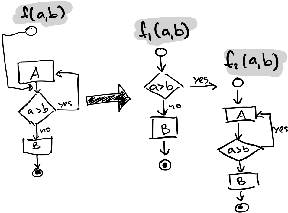
Fig. 1. The function f with a few goto statements inside is translated to two functions, reducing the complexity of the code at the cost of introducing duplication.
