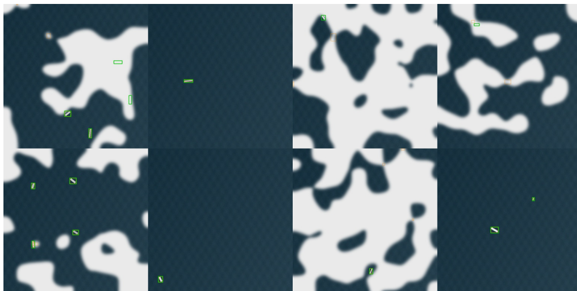
Figure 5 [SIM] — Pre-filter on synthetic tiles: green = ground truth, orange = candidates. On synthetic sea it finds every ship; real imagery is much harder.
