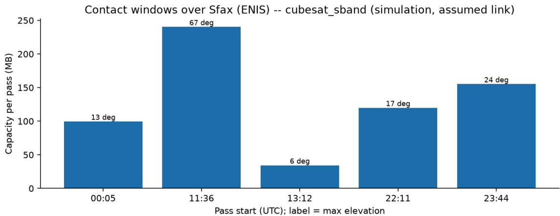
Figure 2 [REAL] — Contact windows of a 500 km sun-synchronous orbit over Sfax ( \geq 5^\circ elevation) and the bytes each pass can carry with the CubeSat S-band link model (assumptions in Appendix A).
