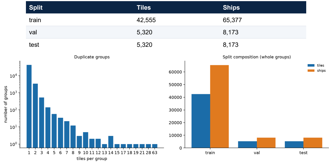
Figure 6 [REAL] — Size of duplicate groups and composition of the leakage-free split.
