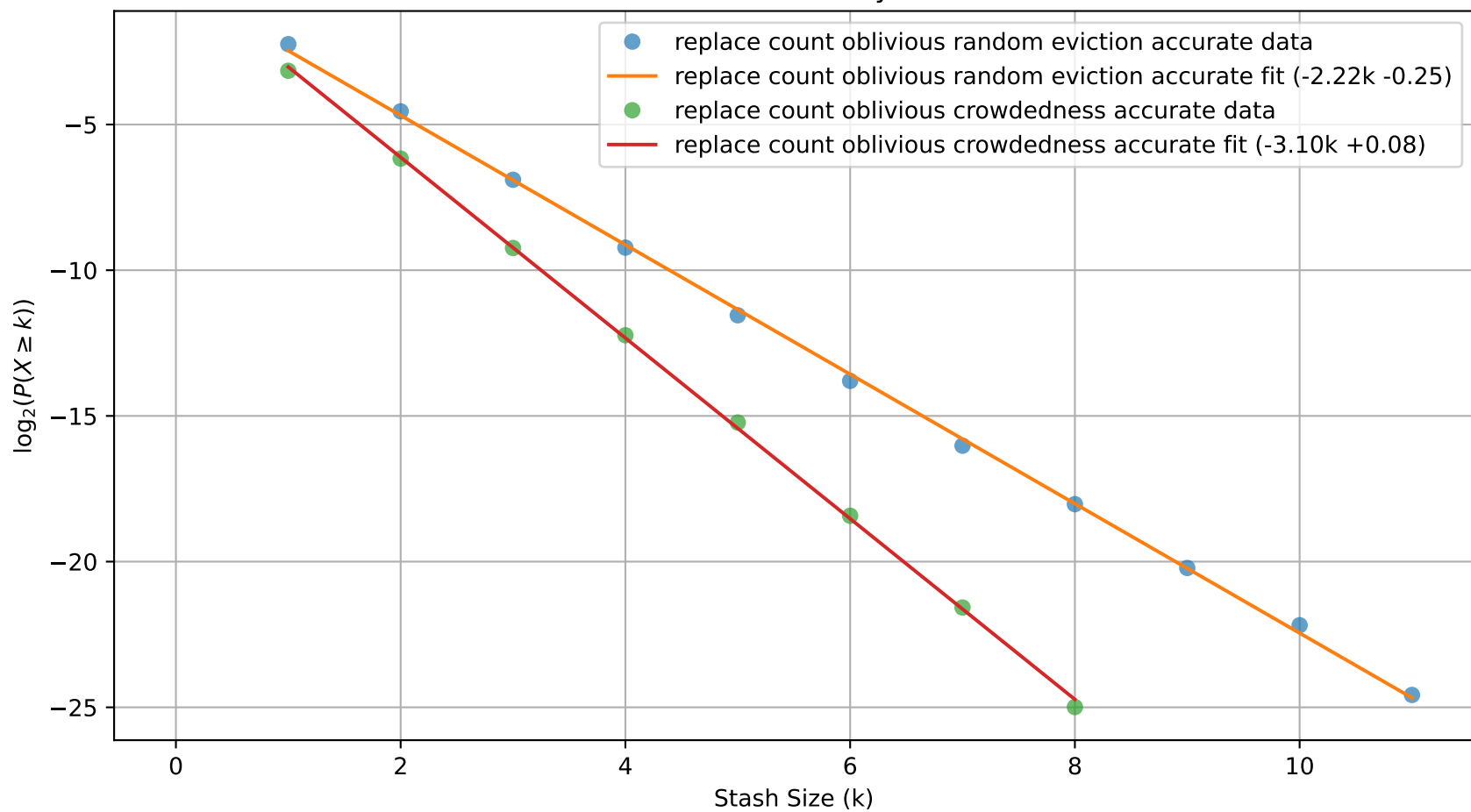
Tail Bound Analysis
