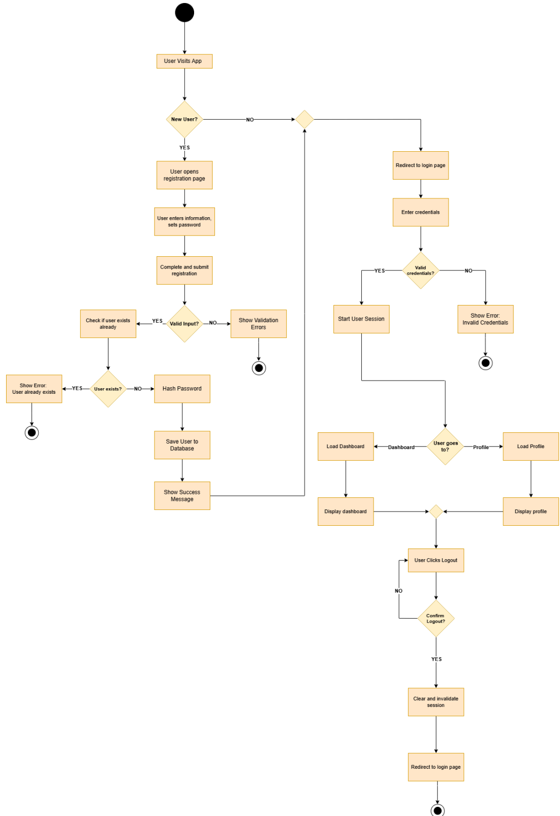
Activity Diagram - Registration, Login, and Logout Flow
