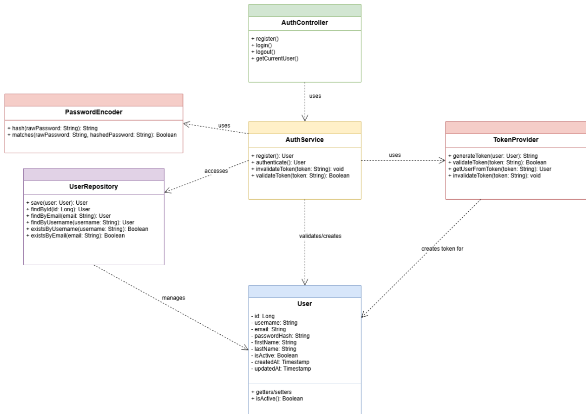
Class Diagram - Authentication System Backend
