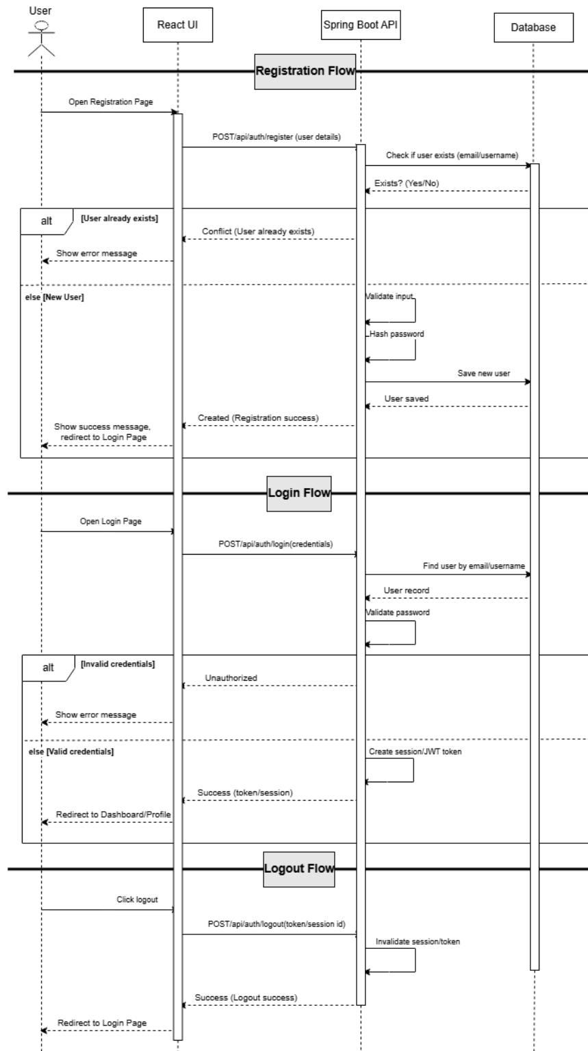
Mini App Register, Login, and Logout Sequence Diagram
