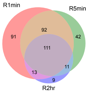
Venn Diagram of Overlap Classes
