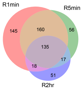
Venn Diagram of Overlap Classes
