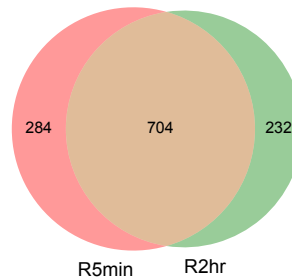
Venn Diagram of Overlap Classes
