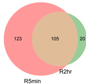
Venn Diagram of Overlap Classes
