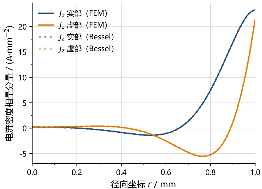
(b) 复数相量分量对照
