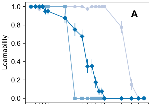
Logistic
