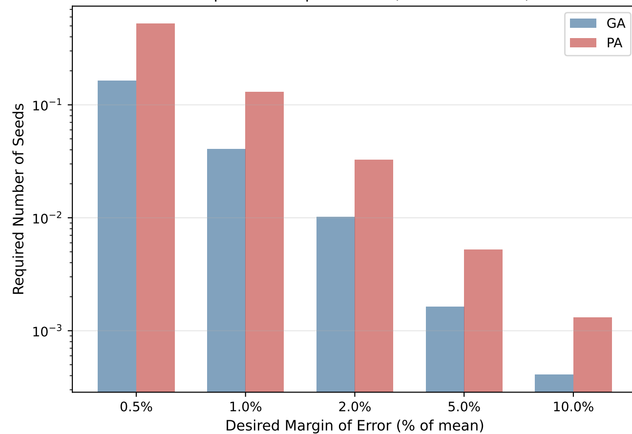
Sample Size Requirements (95% confidence)
