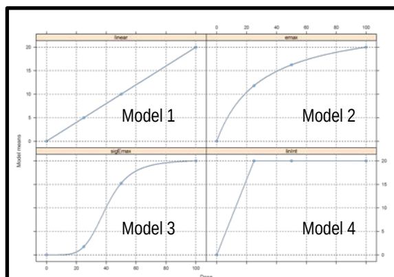
Figure 3: The four proposed models of the Multiple Comparison Procedure and Modelling (MCP-Mod) approach.
