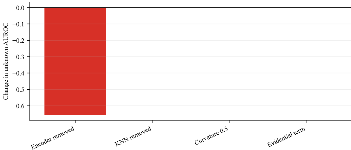
Ablations: only the encoder has a material effect
