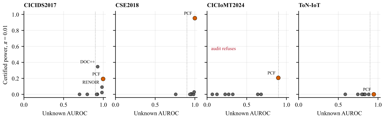
(b) AUROC against certified power at \pi = 0.01 , primary rotation
