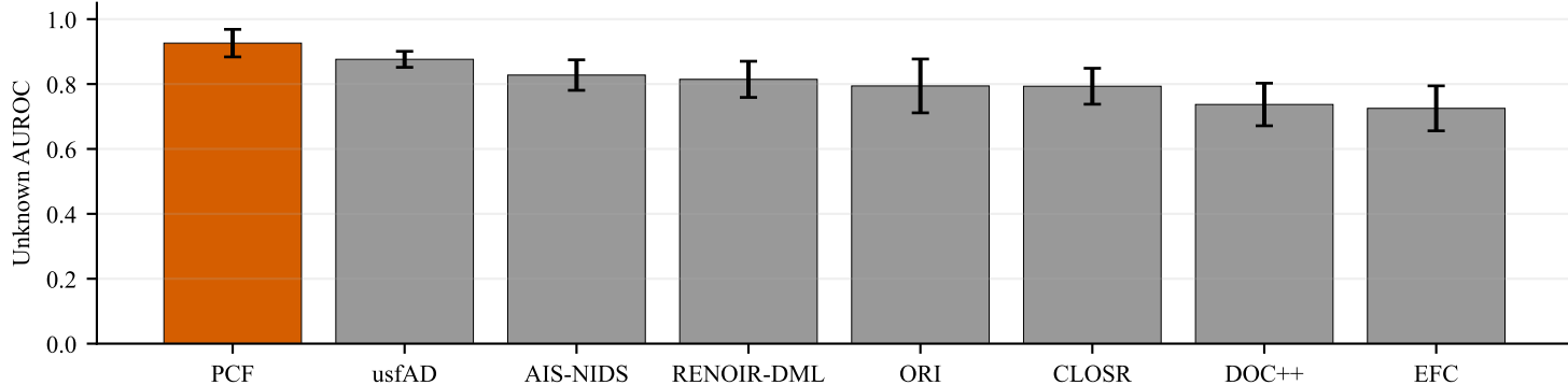
(a) Detector panel: 11 rotations, five seeds
