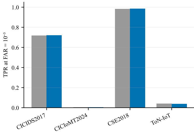
No reliable power gain
