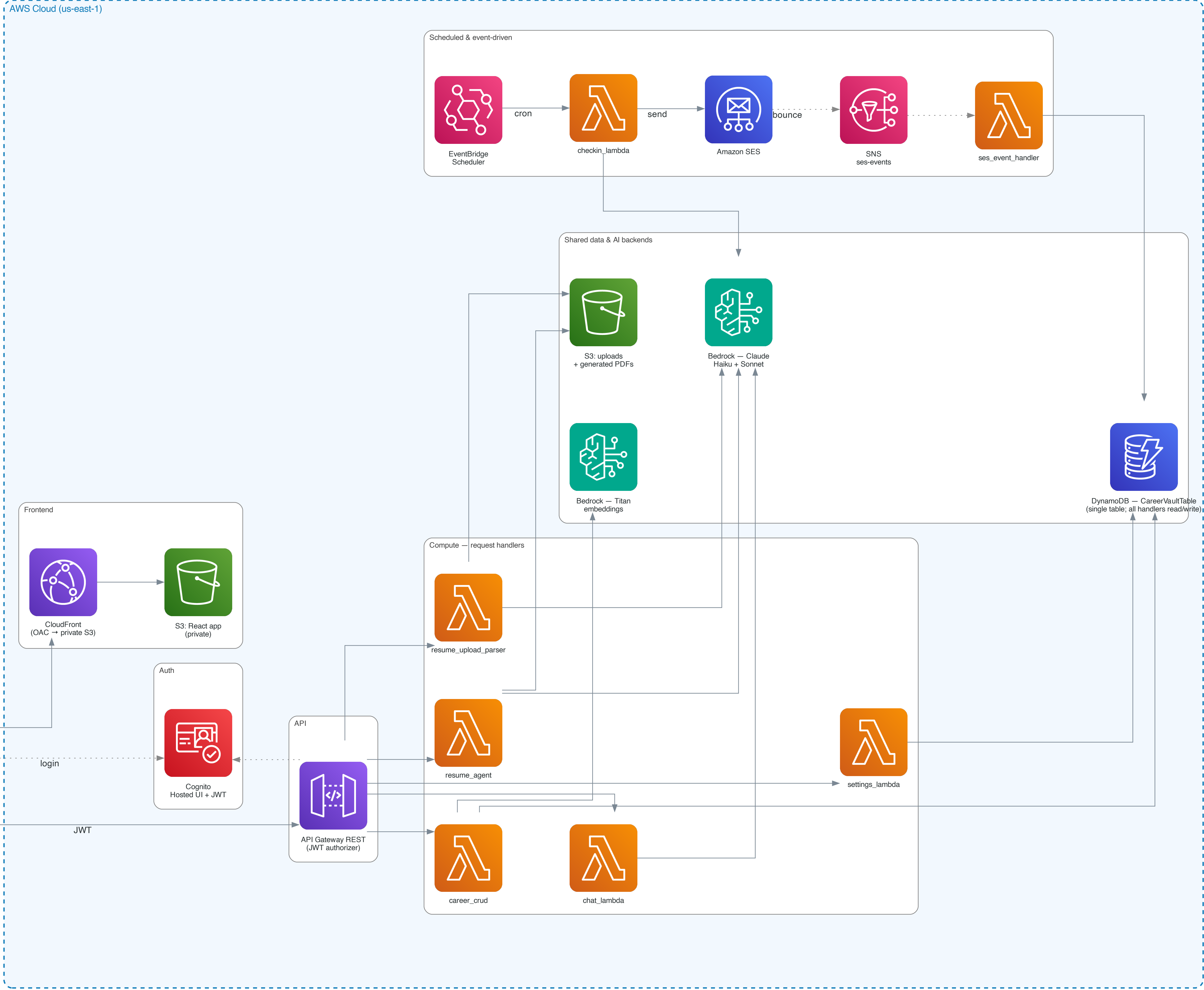
CareerVault v1 — System Architecture
