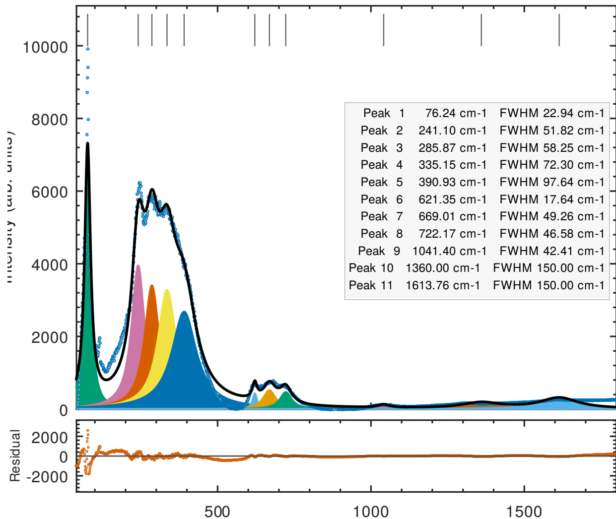
(b) Raman spectrum — Bulk, 300 K | Multi-Lorentzian fit
