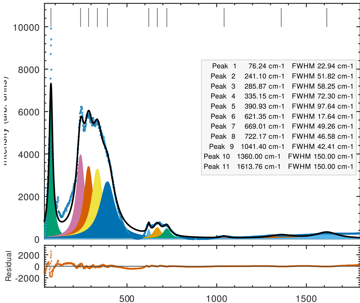
(b) Raman spectrum | Multi-Lorentzian fit
