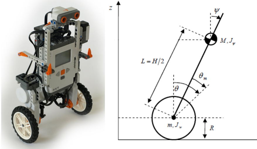
FIGURE 1.4 – Robot Lego segway.
