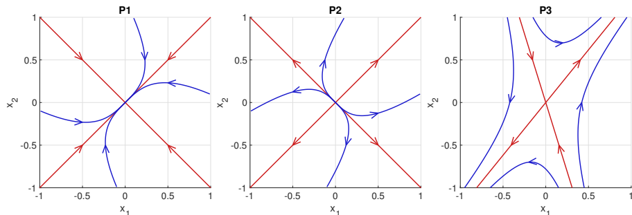
Figure 1 – (Gauche) \lambda_1 < 0, \lambda_2 < 0 . (Milieu) \lambda_1 > 0, \lambda_2 > 0 . (Droite) \lambda_1 \lambda_2 < 0 .
