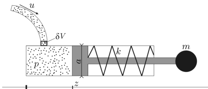
FIGURE 3 – Vérin simple effet.
