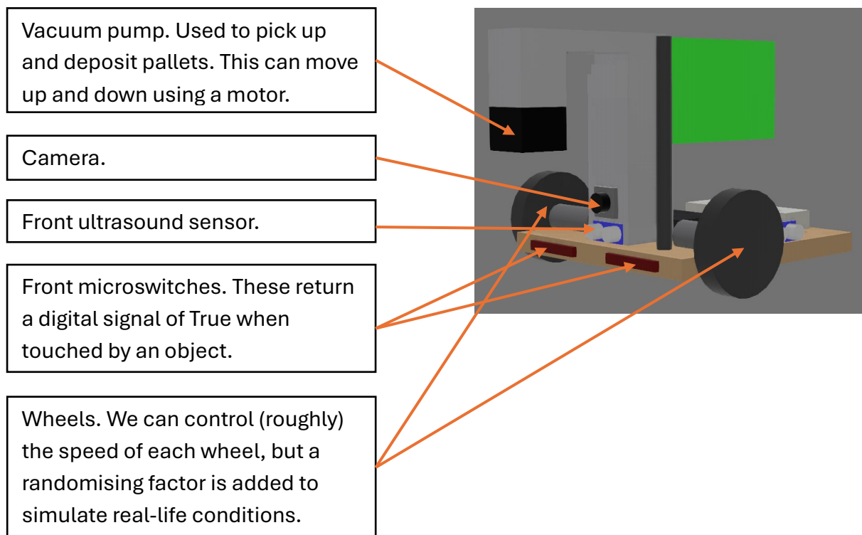
Figure 2: Screenshot of the robot that all teams used, complete with annotations. Only components that we used are annotated.
