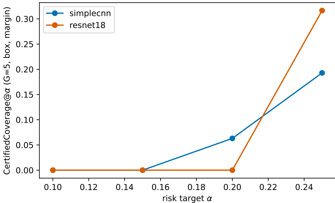
F5 Certified-coverage frontier (cifar10 d=5)
