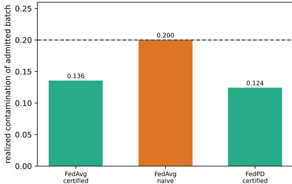
(b) safety: certified \leq alpha (0/N viol.); naive at budget
