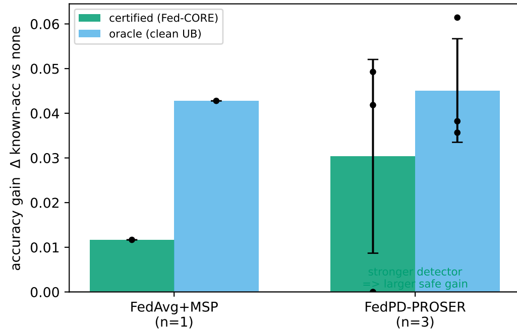
(a) certified self-training gain (alpha=0.20, audit 4x)
