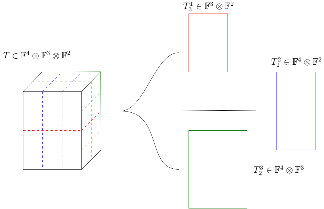
Figure 3: Slicing a tensor T along different modes
