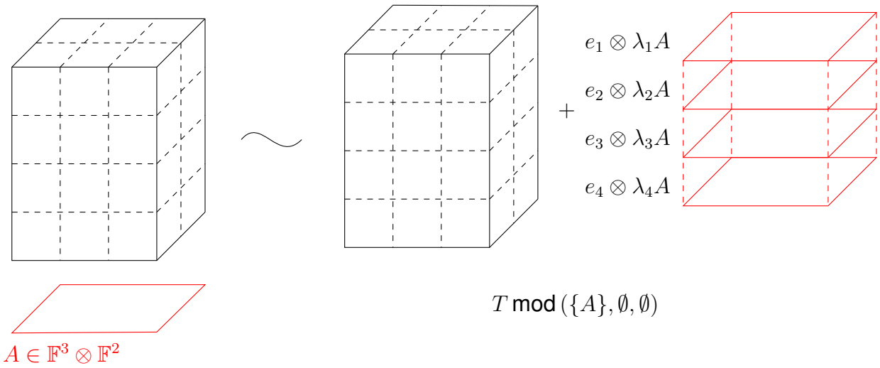
Figure 7: Family generated from a tensor T by a slice A
