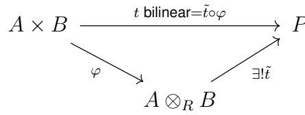
Figure 2: Illustrating a tensor product of R -modules
