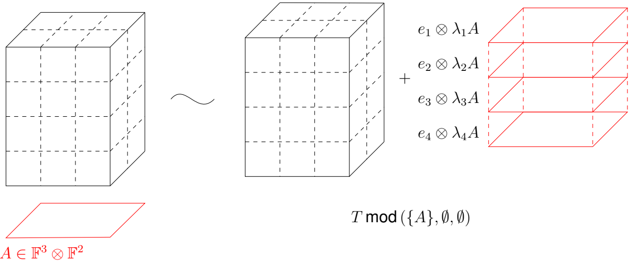
Figure 6: Family generated from a tensor T by a slice A
